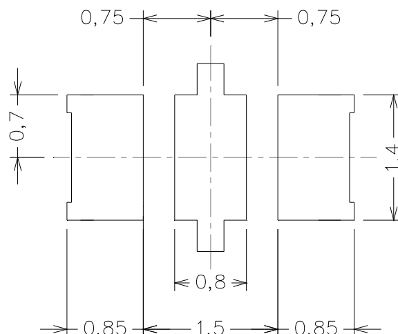
Soldering patterns
